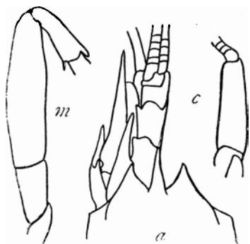
FIG. 2.—SYNALPHEUS PAULSONI. a , FRONTAL AND ANTENNAL REGION; c , CARPOCERITE; m , PORTION OF THIRD FOOT.
