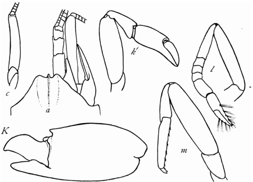
FIG. 47.—SYNALPHEUS TANNERI. a. FRONTAL AND ANTENNAL REGION; c, CARPOCERITE; K, LARGE CHELA; k', SMALL CHELIPED OF FIRST PAIR; l, FOOT OF SECOND PAIR; m, FOOT OF THIRD PAIR.
