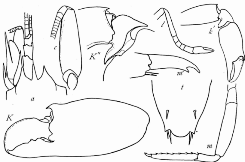
FIG. 9.—SYNALPHEUS APIOCEROS. a , FRONTAL AND ANTENNAL REGION; c , CARPOCERITE; K , LARGE CHELA; K'' , CARPUS OF LARGE CHELIPED; k' , SMALL CHELIPED OF FIRST PAIR; l , FOOT OF SECOND PAIR; m , FOOT OF THIRD PAIR; m' , DACTYL OF THIRD PAIR; t , TELSON.
