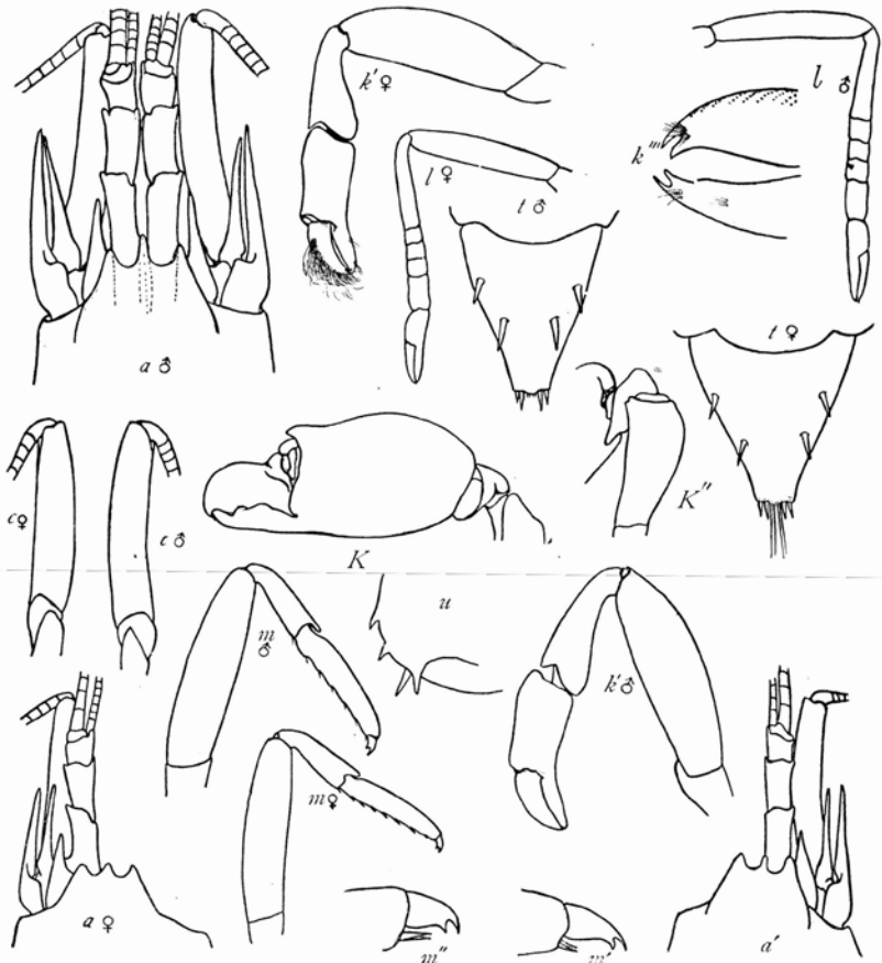
FIG. 44.— SYNALPHEUS HERRICKI . a , FRONTAL AND ANTENNAL REGION, MALE AND FEMALE; a' , FRONTAL AND ANTENNAL REGION OF ANOTHER MALE; c , CARPOCERITE, MALE AND FEMALE; K , LARGE CHELA; K'' , CARPUS AND MEROPODITE OF LARGE CHELA; k' , SMALL CHELIPED OF FIRST PAIR, MALE AND FEMALE; k''' , FINGERS OF SMALL CHELA OF FIRST PAIR; l , FOOT OF SECOND PAIR, MALE AND FEMALE; m , FOOT OF THIRD PAIR, MALE AND FEMALE; m' , DACTYL OF THIRD PAIR OF TYPICAL MALE; m'' , DACTYL OF THIRD PAIR OF ANOTHER MALE; t , TELSON, MALE AND FEMALE; u , UROPOD.
