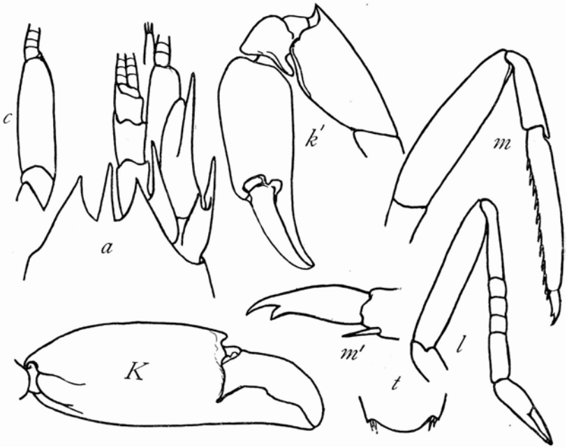
FIG. 1.—SYNALPHEUS LOCKINGTONI. a, FRONTAL AND ANTENNAL REGION; c, CARPOCERITE; K, LARGE CHELA; k', SMALL CHELIPED OF FIRST PAIR; l, FOOT OF SECOND PAIR; m, FOOT OF THIRD PAIR; m', DACTYL OF THIRD PAIR; t, TELSON.
