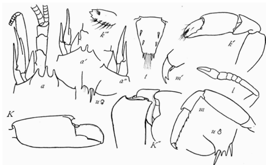
FIG. 52.— SYNALPHEUS PARANEPTUNUS . a , FRONTAL AND ANTENNAL REGION OF TYPE MALE; a' , FRONT AND BASE OF ANTENNÆ OF ANOTHER MALE WITH ANTENNAL SCALE MORE REDUCED; a'' , FRONT AND BASE OF ANTENNÆ OF FEMALE WITH ANTENNAL SCALE ABSENT; K , LARGE CHELA; K'' , MEROPODITE AND CARPUS OF LARGE CHELIPED; k' , SMALL CHELIPED OF FIRST PAIR; k'' , FINGER OF SAME; l , FOOT OF SECOND PAIR; m , FOOT OF THIRD PAIR; m' , DACTYL OF THIRD PAIR; t , TELSON; u , UROPOD, MALE AND FEMALE.
