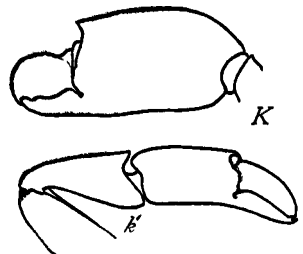
FIG. 46.— SYNALPHEUS HERRICKI DIMIDIATUS . K, LARGE CHELA; k', SMALL CHELIPED OF FIRST PAIR.
