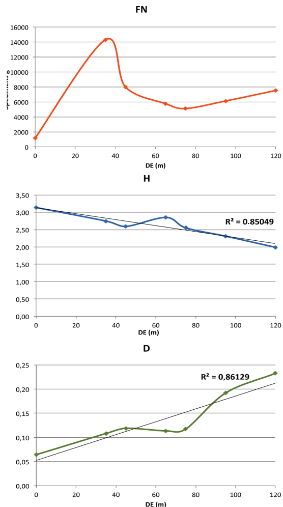
Fig. 4: Values of Foraminiferal Number (FN) Shannon index (H) and Dominance (D) along the cave profile.
