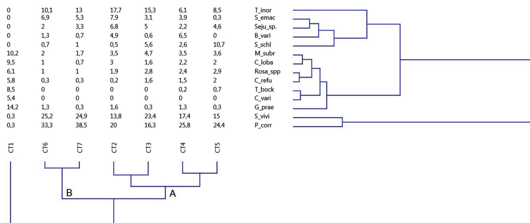
Fig. 6: Two-way (Q-mode and R-mode) Hierarchical Cluster Analysis (HCA) based on relative abundance of commonly occurring foraminiferal species.
