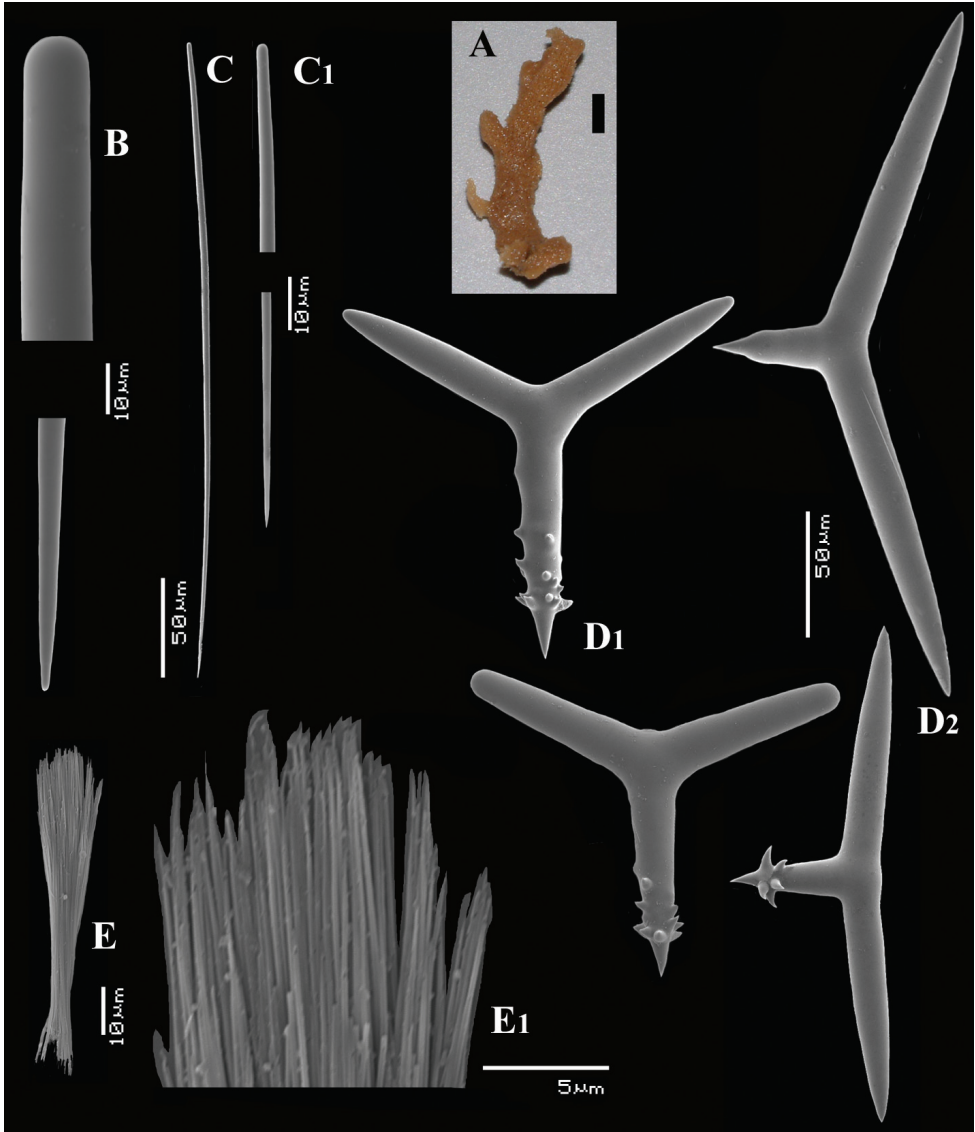
Figure 26. Trikentron africanum sp. n., holotype BMNH 1939.2.20.9, A shape of holotype (scale bar = 1 cm) B details of long thin style C long thin style C1 short thin style D1 details of short thin style D various shapes of polyactines E trichodragma E1 detail of trichodragma.
