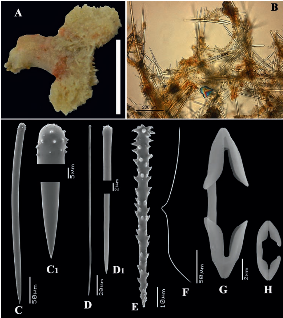
Fig. 23. Clathria (Microcionia) capverdensis spec. nov., A, holotype (ZMA Por. 07380) from the Cape Verde Islands (scale bar = 1 cm), B, cross section of peripheral skeleton (scale bar = 200 μm), C-H, SEM images of the spicules, C-C1, structural style and detail of head and pointed end, D-D1, ectosomal subtylostyle and detail of head and pointed end, E, echinating acanthostyle, F, accolada tox, G, larger category of palmate isochela, H, smaller category of palmate isochela.
