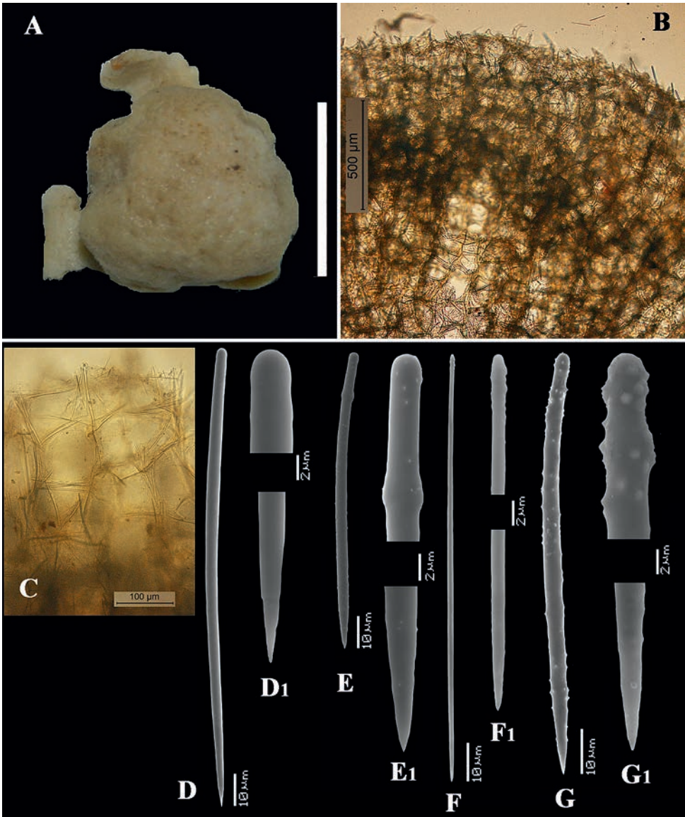
Fig. 43. Antho (Antho) nuda spec. nov., A, holotype (ZMA Por. 06911) from the Cape Verde Islands (scale bar = 1 cm), B, cross section of skeleton (scale bar = 500 µm), C, detail of skeleton (scale bar = 100 µm), D-G, SEM images of spicules, D-D1, long ectosomal smooth style and detail of head and pointed end, E-E1, small choanosomal smooth style with detail of head and pointed end, F-F1, ectosomal subtylostyle with detail of head and pointed end, G-G1, acanthostyle from the choanosomal reticulation and detail of head and pointed end.
