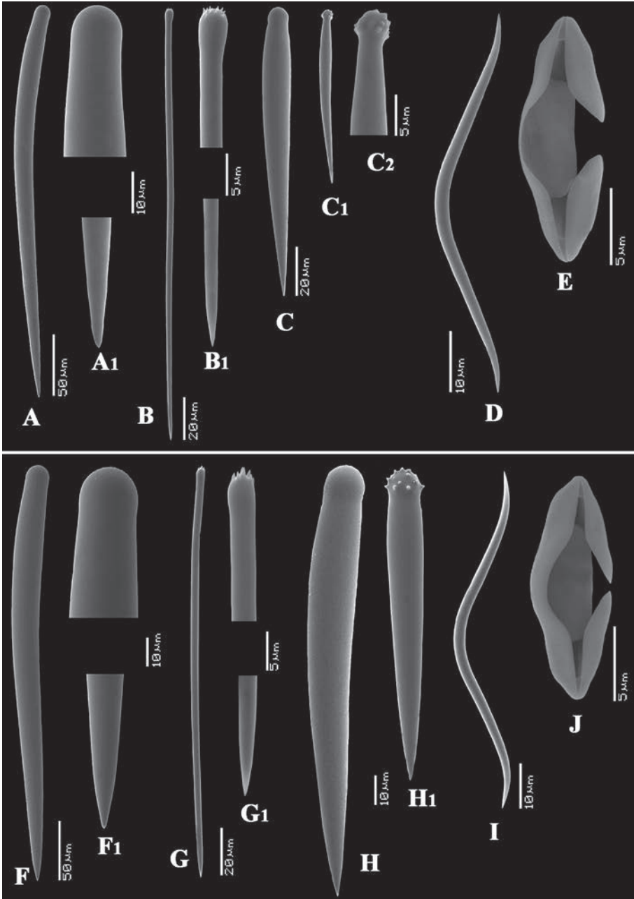
Fig. 4. Clathria (Clathria) hjorti comb. nov., A-E, SEM images of the spicules of holotype (ZMUB 25643), A, structural style, A1, details of head and pointed end, B, subtylostyle, B1, detail of head and pointed end, C-C1, larger and smaller echinating styles, C2, detail of head of C1, D, tox, E, cleistochela, F-G, SEM images of the spicules of Mauritania specimen (ZMA Por. 06605), F, structural style, F1, details of head and pointed end, G, subtylostyle, G1, detail of head and pointed end, H-H1, larger and smaller echinating styles, I, tox, J, cleistochela.
