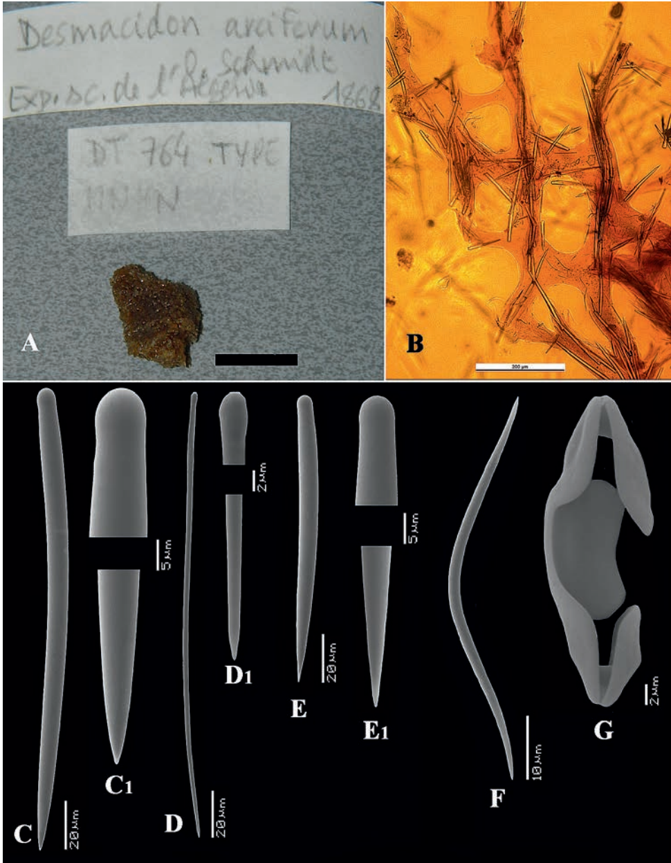
Fig. 7. Clathria (Clathria) arcifera (Schmidt, 1868 as Desmacidon ) comb. nov. from Algeria, A, habitus of remaining fragment of holotype (MNHN D.T.764) and labels (scale bar = 1 cm), B, cross section of peripheral skeleton (scale bar = 200 µm), C-G, SEM images of spicules, C-C1, structural style and detail of head and pointed end, D-D1, ectosomal subtylostyle and detail of head and pointed end, E-E1, echinating style and detail of head and pointed end, F, tox, G, cleistochela.
