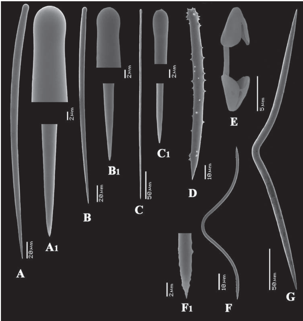
Fig. 45. Antho (Antho) paradoxa (Babič, 1922), specimen (RMNH Por. 3853) from Madeira, assigned neotype status herein, SEM images of spicules, A-A1, long ectosomal smooth style and detail of head and pointed end, B-B1, small choanosomal smooth style with detail of head and pointed end, C-C1, ectosomal subtylostyle with detail of head and pointed end, D, acanthostyle from the choanosomal reticulation, E, palmate isochela, F-F1, wing-shaped toxas and detail of spined ending, G, giant oxete tox.
