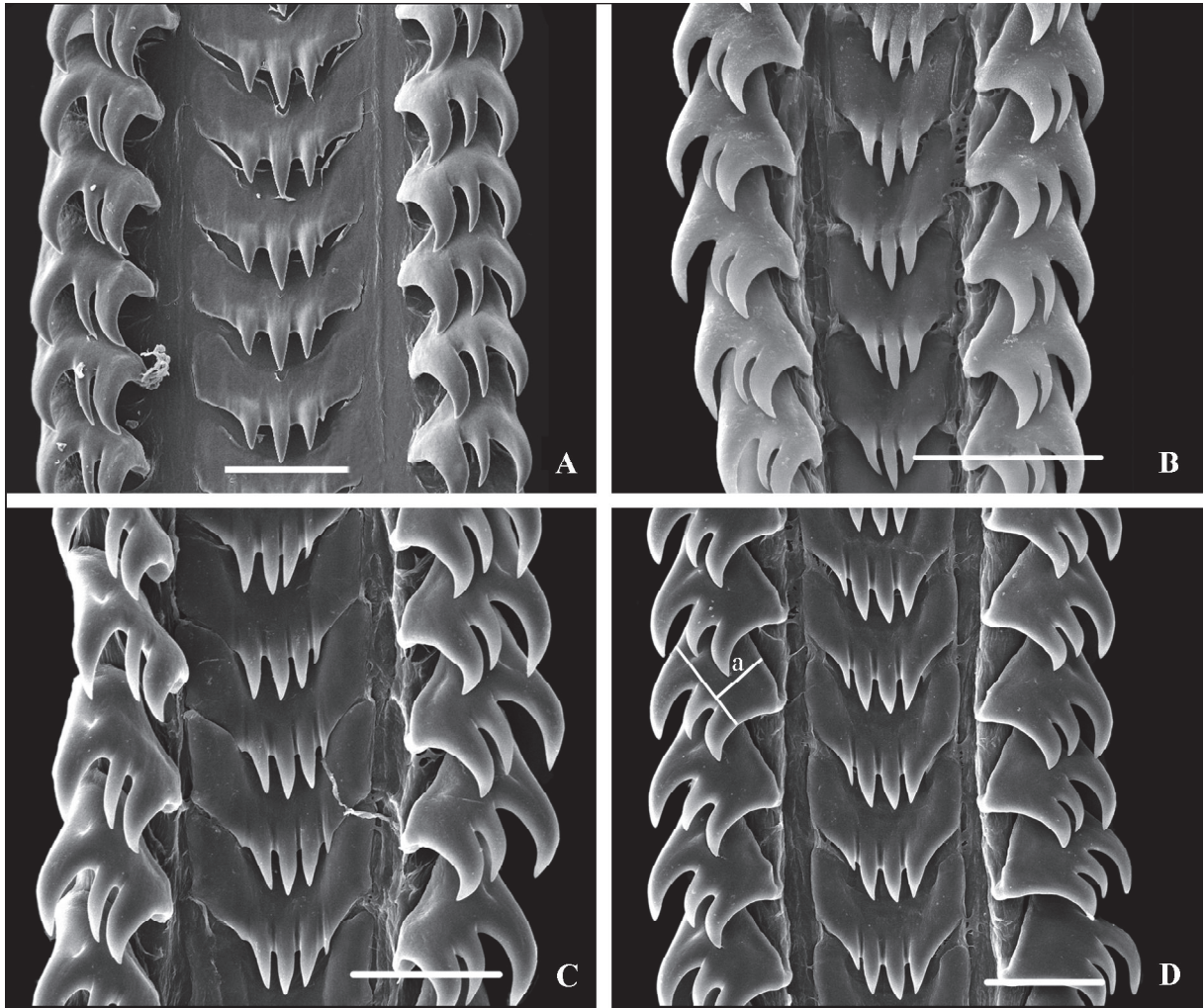
FIG. 2. Radulae of Retimohnia . A. Paralectotype of Mohnia frielei (shell on Fig. 1B). B-D. R. hondoensis . B, no. 1. C, no. 2. D, no. 3 (shells on Fig. 1D-F, anatomy of no. 1 on Fig. 5); a height of basal part of lateral tooth. Scale bar = 50 \mu m.
