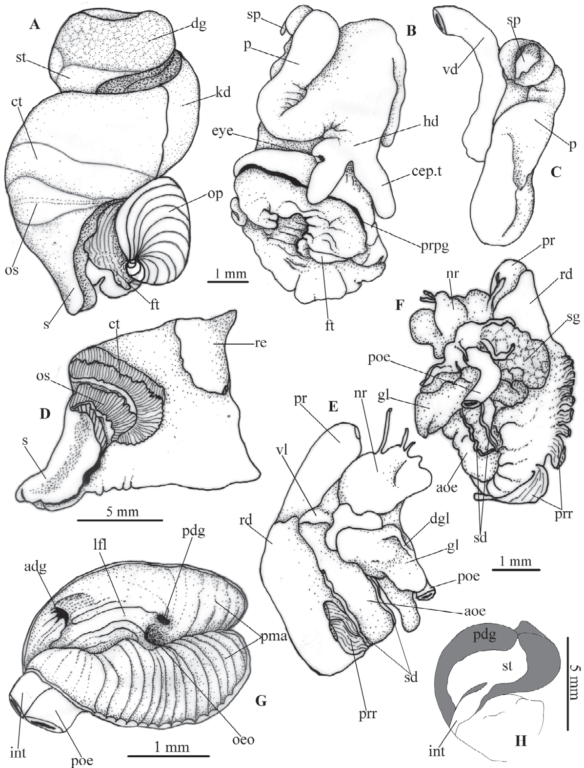
FIG. 19. Anatomy of holotype of Retimohnia mcleani sp. nov. (shell on Fig. 18A, radula on Fig. 20A). A. Soft body front view. B. Cephalopodium, dorsal view. C. Distal parts of male reproductive system. D. Mantle. E. Foregut, right lateral view (salivary glands removed). F. Foregut, left ventral lateral view. G. Stomach, opened dorsally. H. Stomach general view.
