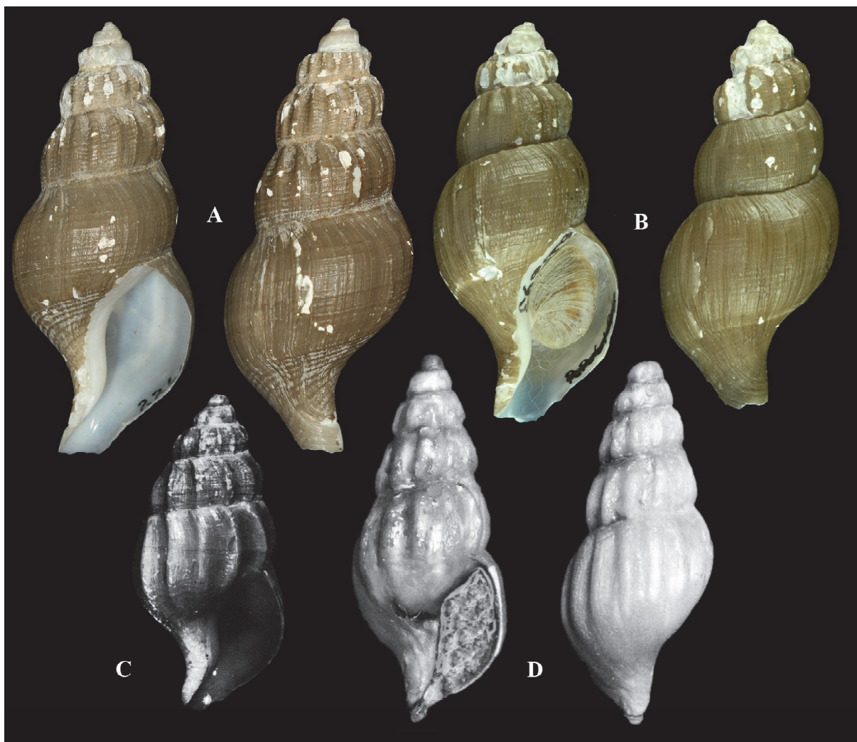
FIG. 24. Shells of Retimohnia . A. Holotype of R. robusta (Dall, 1913) USNM 635693, 54°11'30"N, 167°25'W, 1805 m, 36.5 mm. B. Paratype of R. robusta USNM 226196, 54°11'30" N, 167°25'W, 1805 m, 34.1 mm. C. R. caelata (Verrill et Smith, 1880), SE Delaware Bay, 1492 m, 17.6 mm (photo taken from Bouchet, Warén, 1985). D. Holotype of R. acadiana García, 2008 ANSP 418029, 27°46.904'N 91°30.286'W, 546-555 m, H 20.9 mm. Shells not to scale.
