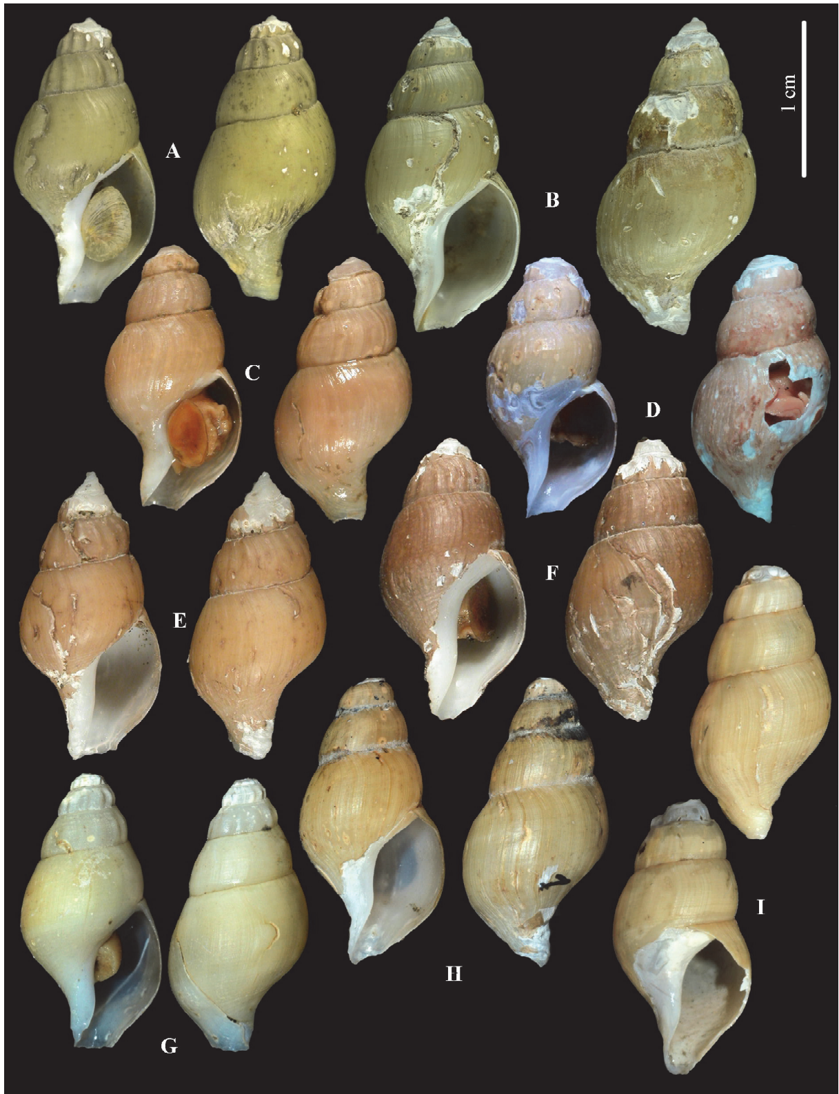
FIG. 11. Shells of Retimohnia clarki . A. Lectotype, USNM 110497, eastern Kamchatka, 52°37'30"N 158°50'E, 1247 m, H 21 mm. B. Holotype of L. clementinus Dall, 1919, USNM 209110, North of California, between Santa Catalina and San Clemente Islands, 1196-1287 m, H 20.5 mm (radula on Fig. 13A). C. No. 1, 57°51'N, 148°57'W, Alaska Bay, near Kadiak Lake, 1350-1340 m, H 16.7 mm (radula on Fig. 13B). D. No. 2, southern coast of Sakhalin, 1450-1530 m, H 17.1 mm (radula on Fig. 13C). E-F. Nos. 3-4, Pacific coast of Kamchatka, Kronotsky Bay, 940-1015 m, H 17.6 mm and 17.3 mm respectively (anatomy of no. 3 on Fig. 12, radula on Fig. 14A, radula of no. 4 on Fig. 14B). G-H. Nos. 5-6, 53°46'N, 163°41'W, Aleutian trench, 1100-830 m, H 15.6 mm and 18.1 mm respectively (radulae on Fig. 14 C-D). I. No. 7, Aleutian trench, 53°43'N, 163°35.7'W, 1690-1740 m, H 17.0 mm (radula on Fig. 14 E-F). Scale bar 10 mm.
