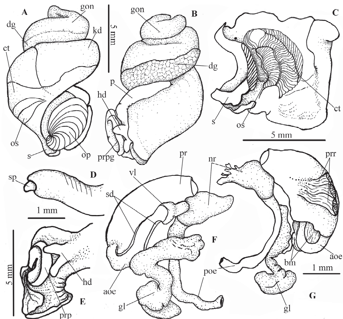
FIG. 8. Anatomy of Retimohnia micra no. 2 (shell on Fig. 7D, radula on Fig. 9B). A-B. Soft body. C. Mantle. D. Penis. E. Head-foot. F. Foregut right lateral view (salivary glands removed). G. Foregut left lateral view (salivary glands removed).
